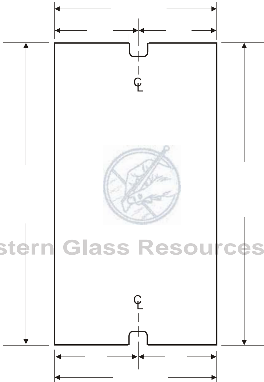
No. TP1-TRANSOM PANEL - (Fixed or Moveable)
