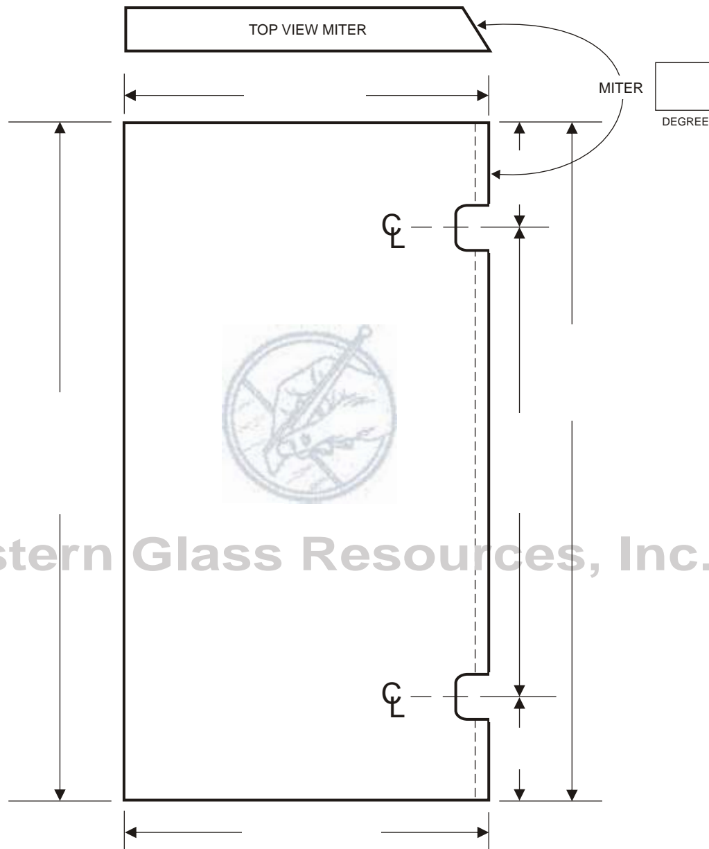
No.FM1 FIXED PANEL - (Miter and Hinge Cutouts on Right Side)
