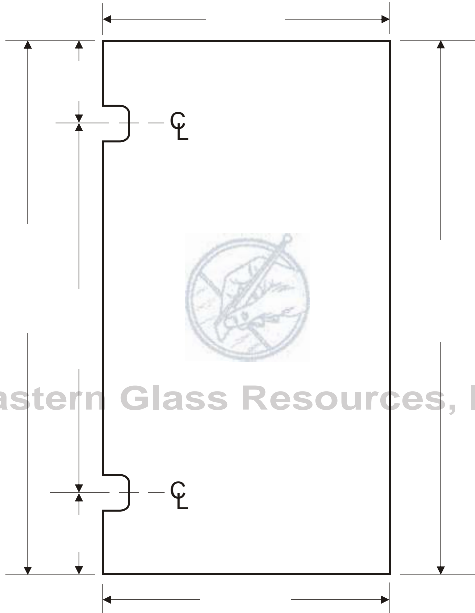
No.FH2 FIXED PANEL - (Hinge Cutouts on Left Side)
