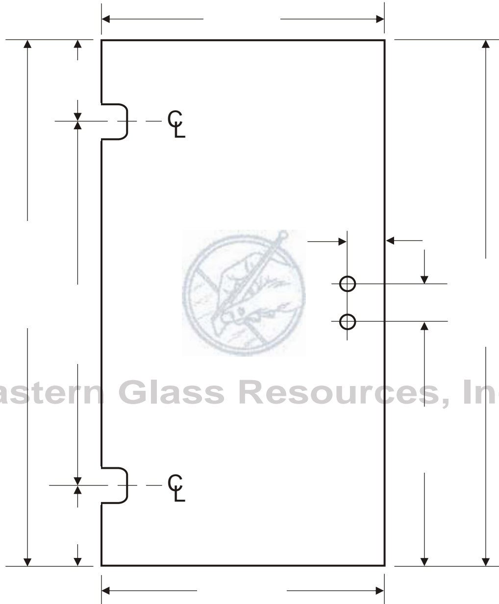
No.DS1 Door Glass Template - (Side Mount, Hinge Left)
