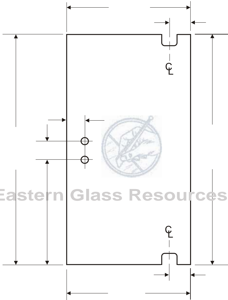
No.DP2 Door Glass Template - (Top and Bottom Mount, Hinge Right)
