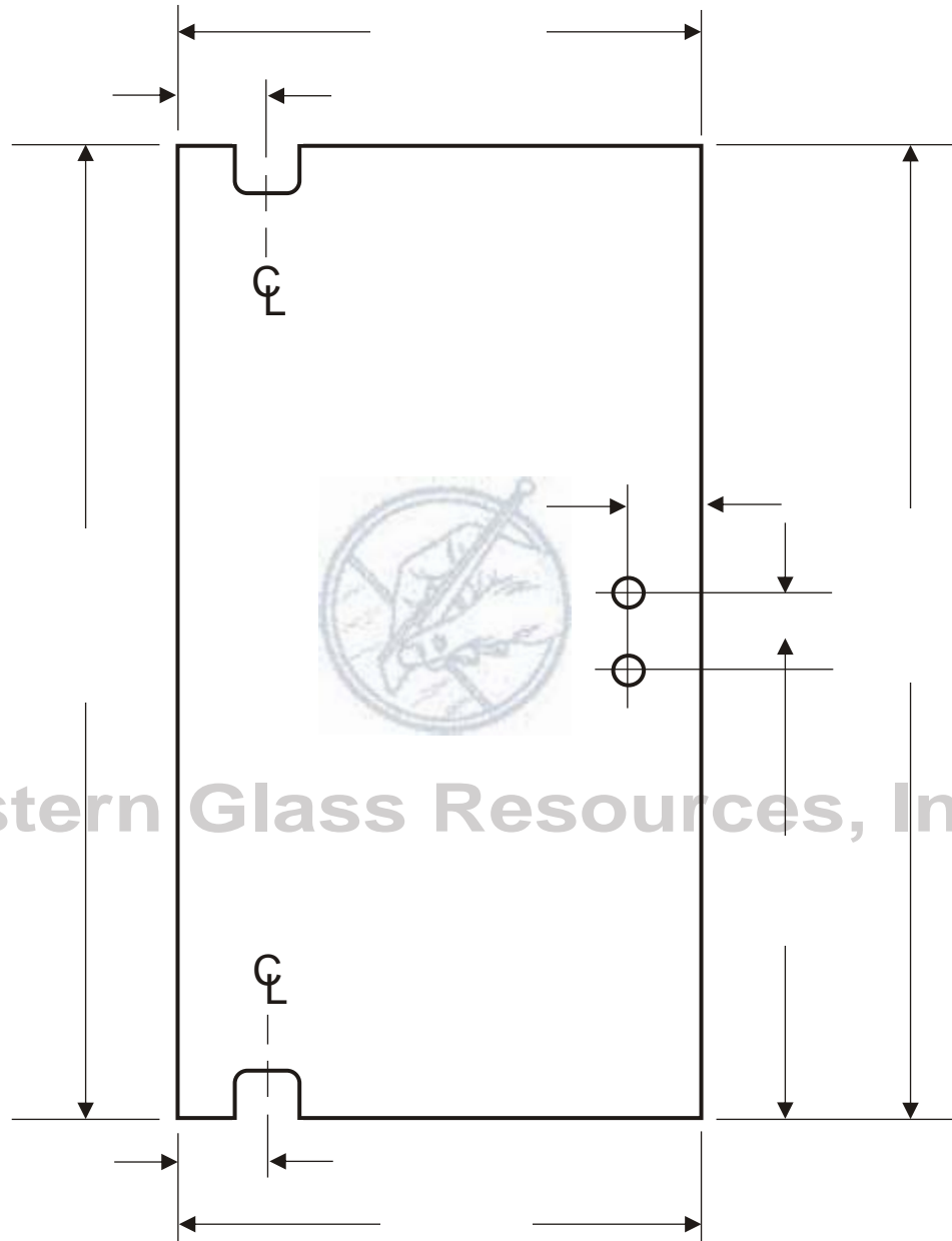
No.DP1 Door Glass Template - (Top and Bottom Mount, Hinge Left)
